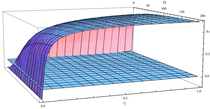
Figure 1: \Delta for \gamma \in [0, 1] and n \in [3, 200] .
