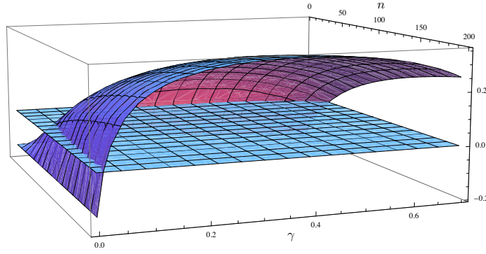
Figure 2: \tilde{\Delta} for \gamma \in [0, 0.7] and n \in [3, 200] .
