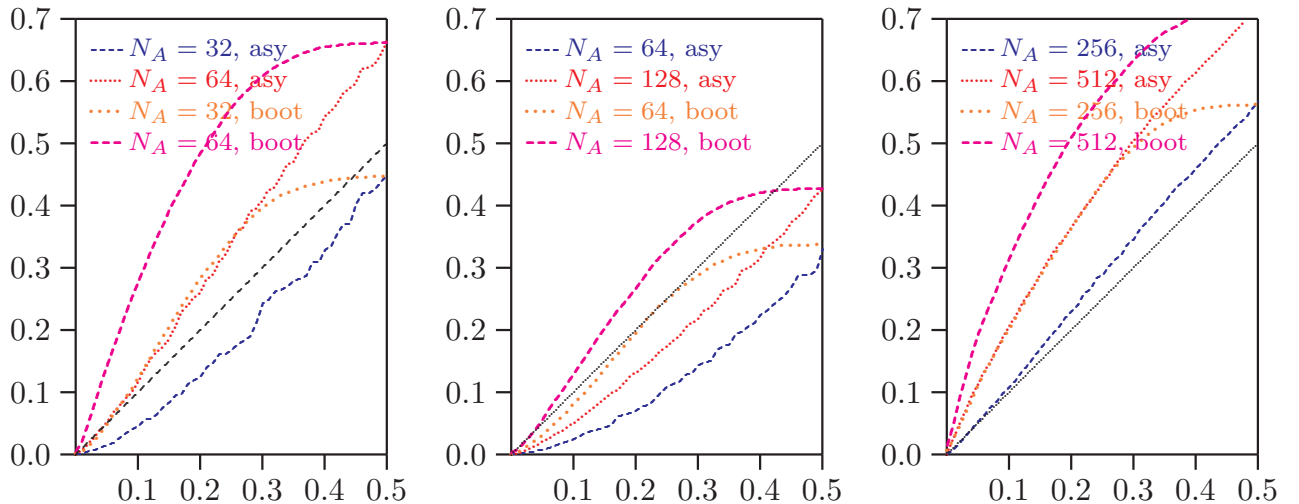
Figure 5: Power curves
