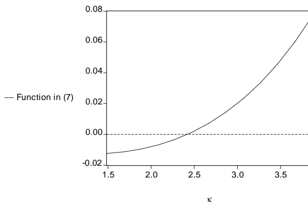
Figure 5: \hat{\Psi}_T(\kappa) for wholesale price.
