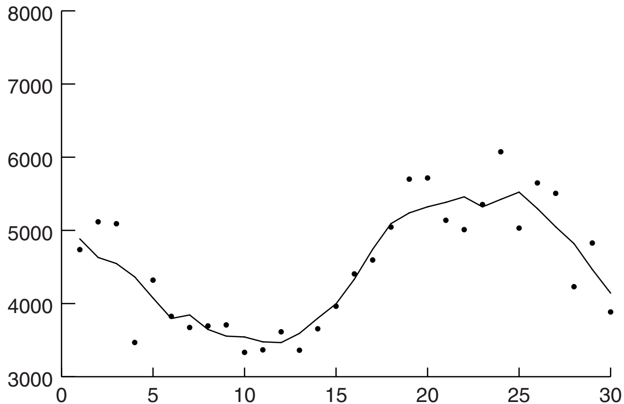
Simple 5-term moving-average of the strike data from Figure 1.6
